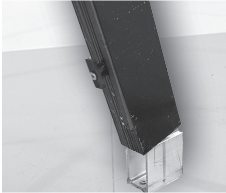
IV.9. Install vertical profiles as shown in the photo.
