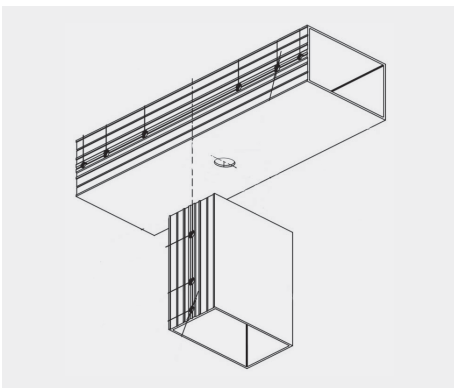
IV.12. Align the top horizontal beam with the reference line on the ceiling. Mark the center of the vertical beam on the bottom side of the top horizontal beam to drill the holes. The holes should be located in the places the vertical profile meets horizontal beam as shown in the photo.
